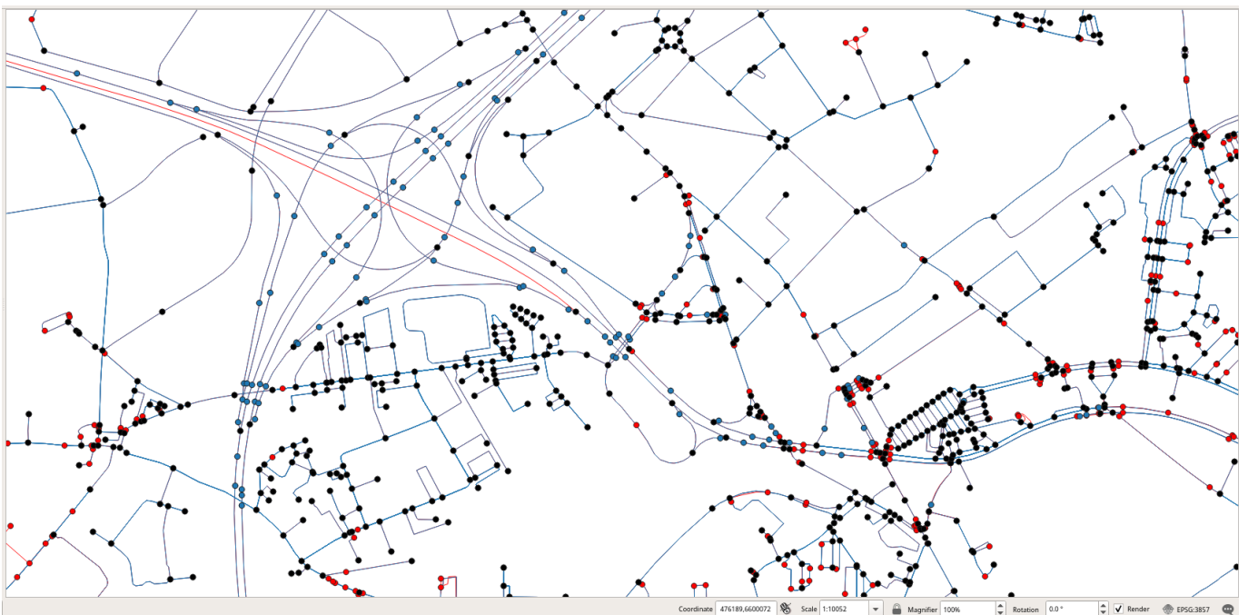
Figure 2.9: Comparison of the nodes obtained by contracting the graph (in black), before contraction (in blue), and those obtained by osm2pgrouting (in red).
