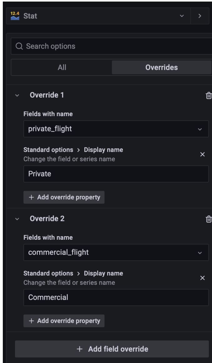
Figure 3.12: Override options for panel with multiple queries
