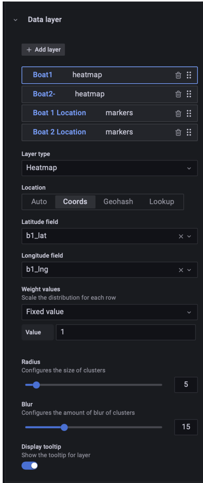
Figure 2.14: Multiple layers in data layers dialogue box
