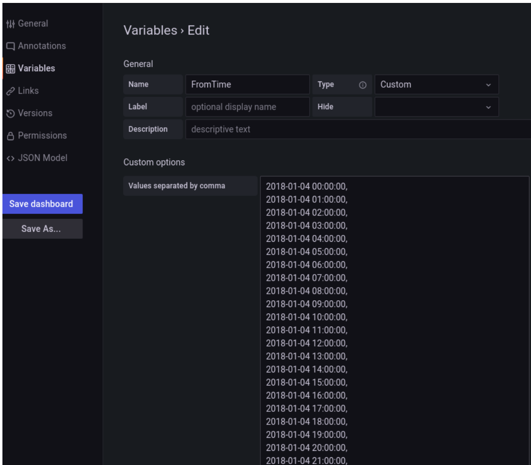
Figure 2.19: Creating user-defined list of custom variables
