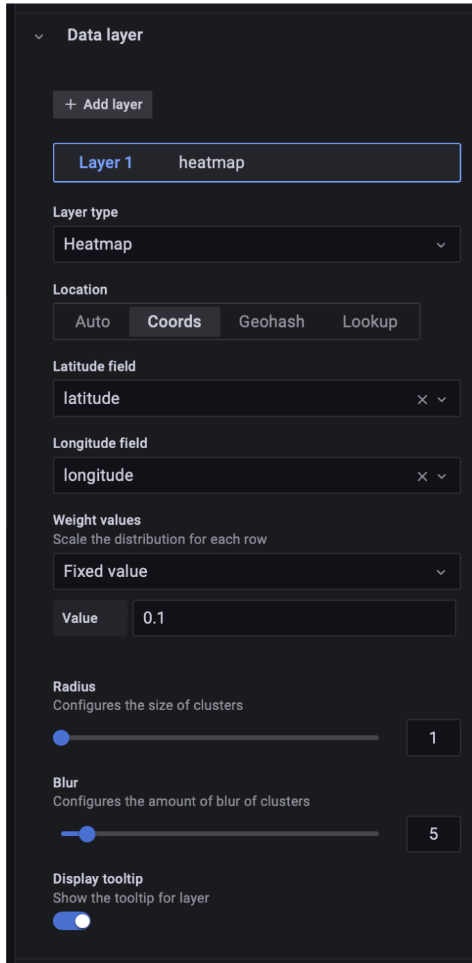
Figure 2.10: Setting up heat-map in data layer dialog box
